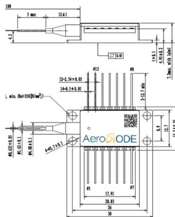
Dimensions are in mm
